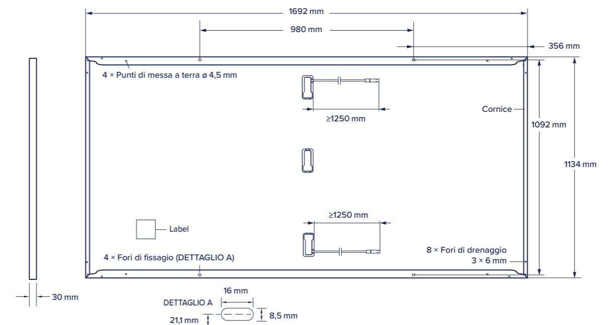
Fig. 1: Dimensioni d'ingombro (in mm) e componenti per Q.PEAK DUO M-G11 Q.PEAK DUO BLK M-G11 Q.PEAK DUO M-G11+ Q.PEAK DUO BLK M-G11+
